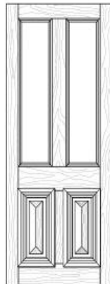
2 LIGHT 2 PANEL CRICKET BAT ENTRY DOOR 820 x 2040 x 40
