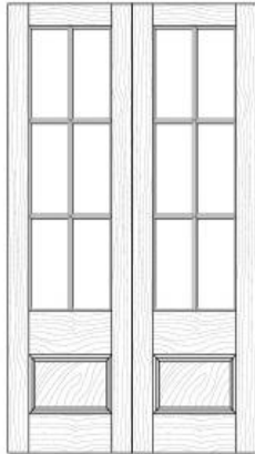
6 LIGHT 1 PANEL GLAZED FRENCH DOOR 620 / 720 / 820 x 2040 x 40
