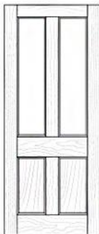
2 LIGHT 2 PANEL 820 x 2040 x 40
