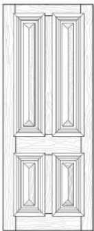
4 PANEL CRICKET BAT ENTRY DOOR 820 x 2040 x 40
